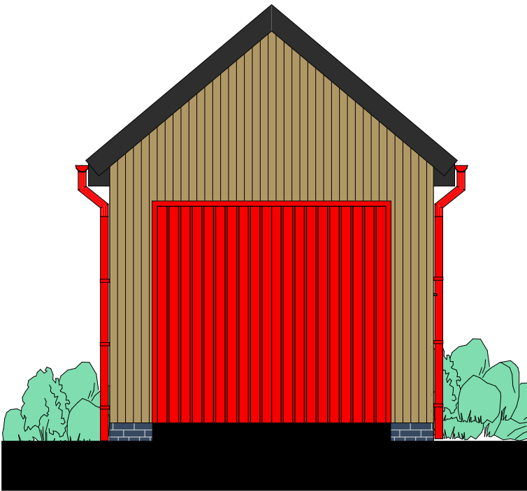
Left Elevation
